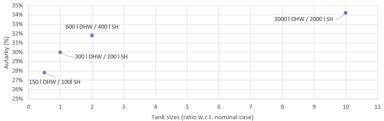
Figure 13 : autarky as a function of tank sizes
