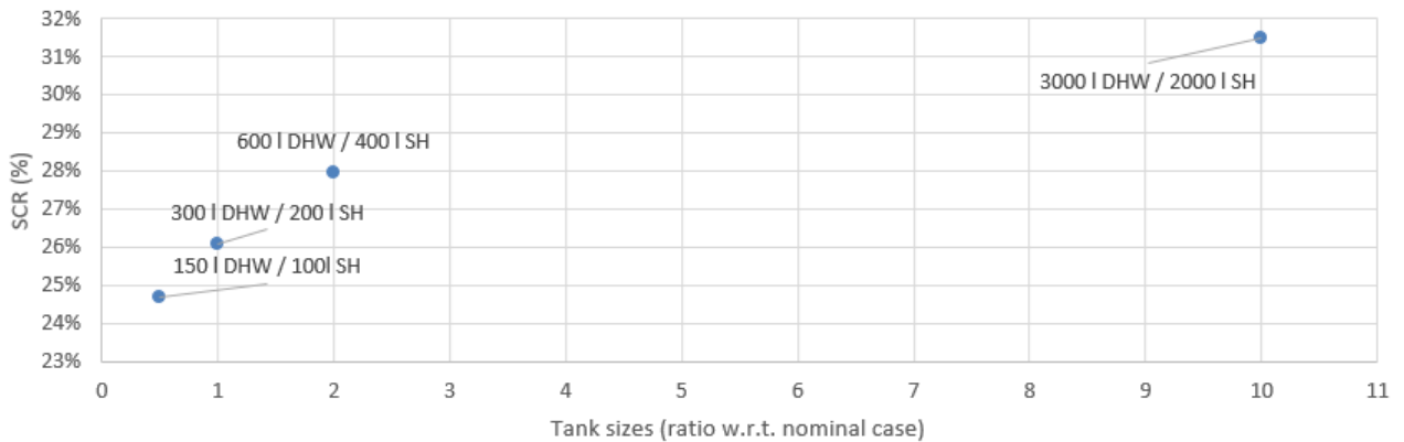
Figure 12 : SCR as a function of tank sizes
