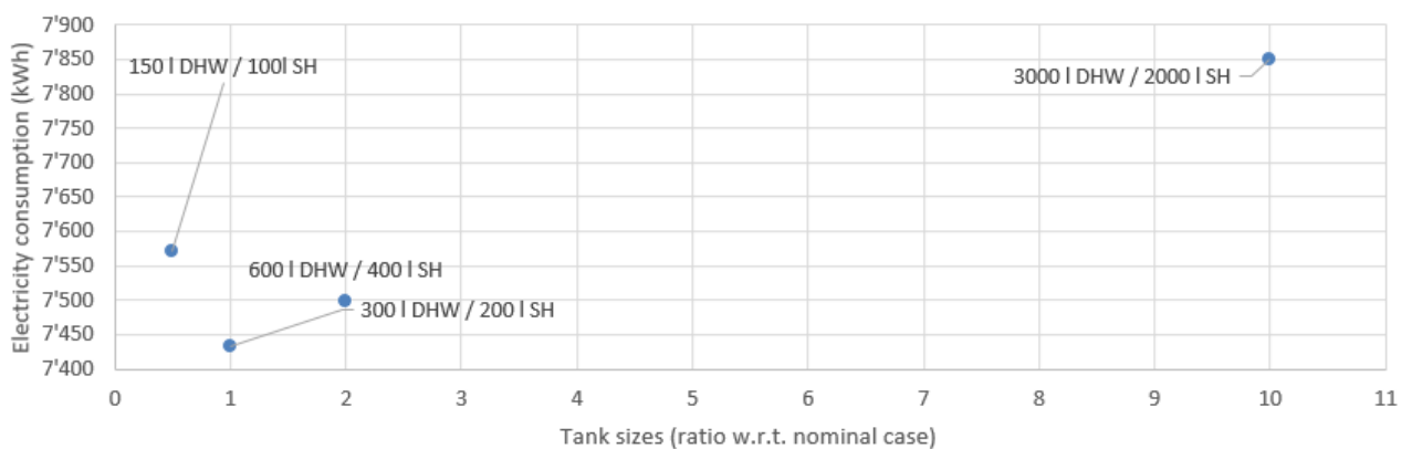
Figure 14 : total electricity consumption as a function of tank sizes
