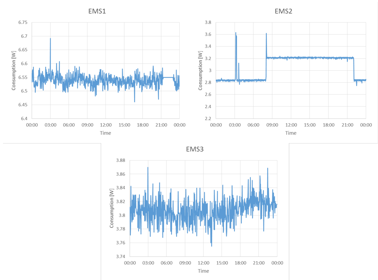
Figure 7 : Daily energy consumption measured for each EMS.
